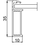
B-B 10: 1
