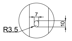
D-position Mounting Hole
