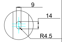
5:1 C-position Mounting Hole
